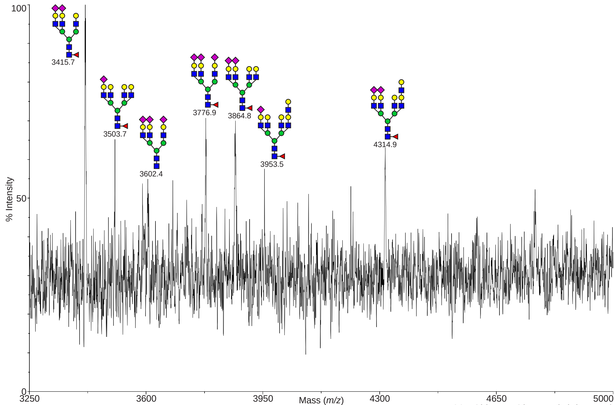
A007 Skin - N-Glycans (High Mass)
