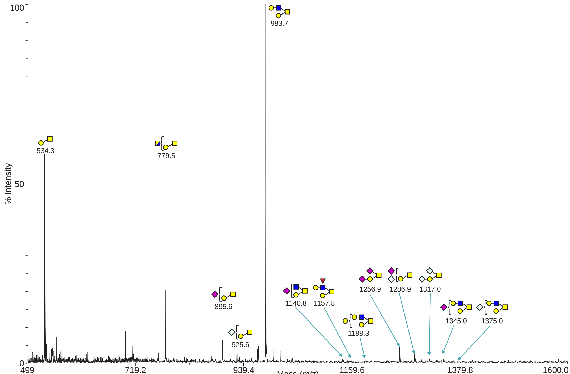
FucTIV & FucTVII Double Knockout Testis - O-Glycans
